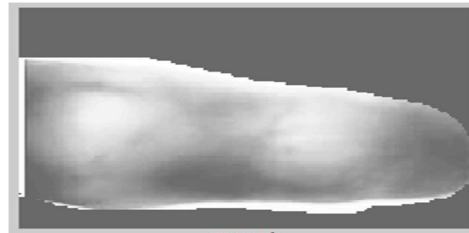
Fig.5 Enhanced image
